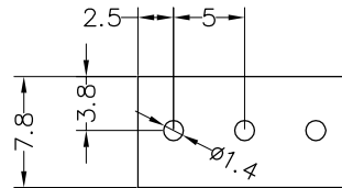
Recommended P.C.B Layout(Top Side)
